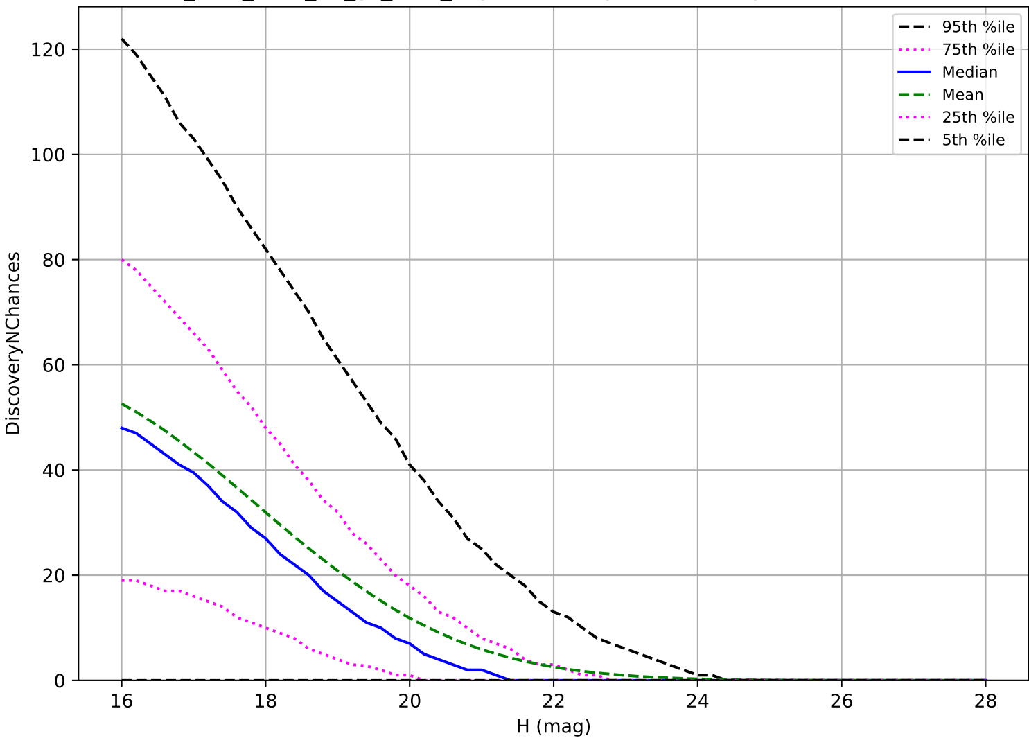
too_elab_r256_d3_gz_v3.4_10yrs: NEO 3 pairs in 15 nights detection loss
