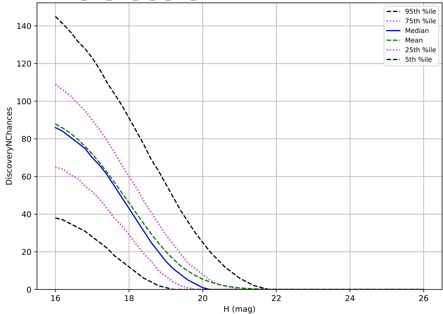
too_elab_r256_d3_gz_v3.4_10yrs: MBA 3 pairs in 15 nights detection loss
