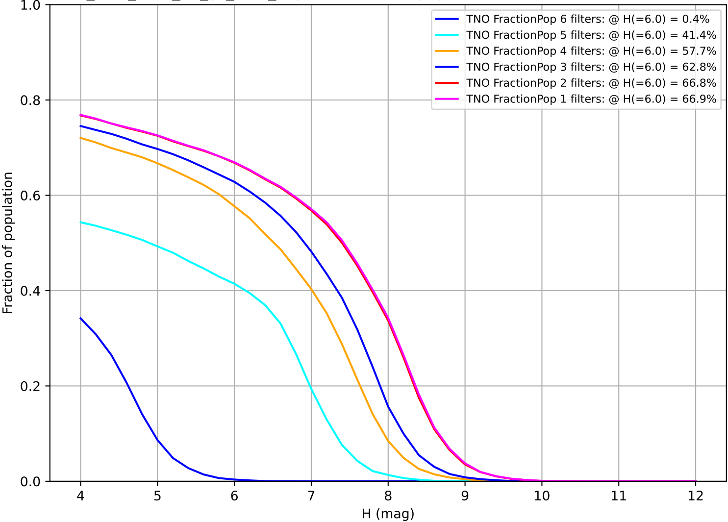
too_elab_r256_d3_gz_v3.4_10yrs: Fraction of population with colors in X filters TNO
