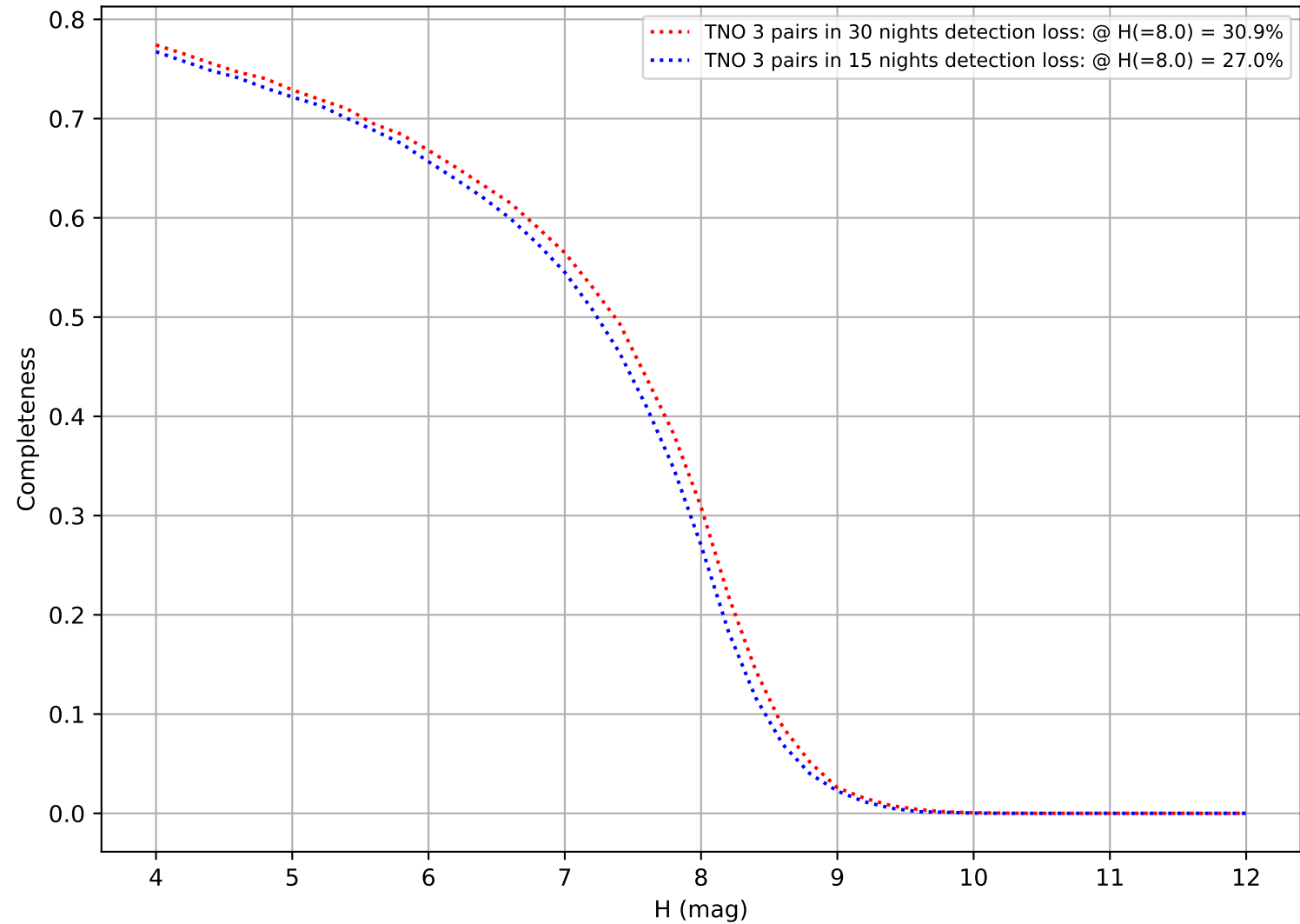
too_elab_r256_d3_gz_v3.4_10yrs: DifferentialCompleteness
