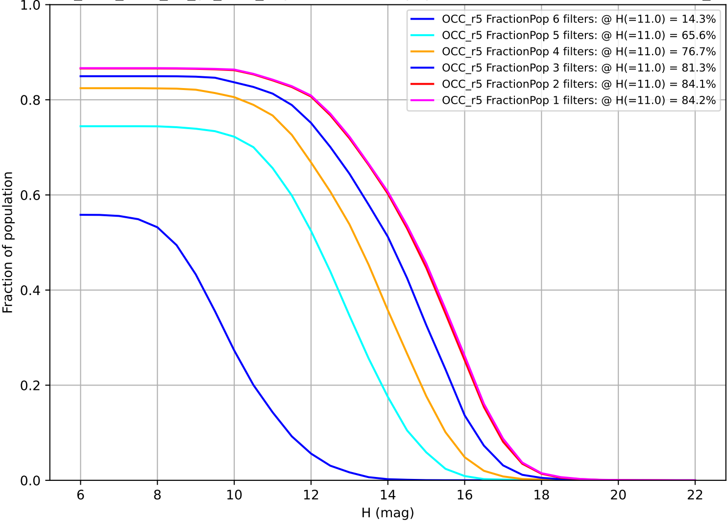
too_elab_r256_d3_gz_v3.4_10yrs: Fraction of population with colors in X filters OCC_r5
