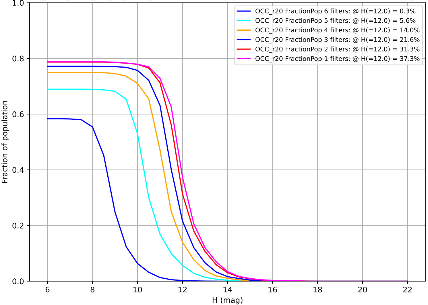
too_elab_r256_d3_gz_v3.4_10yrs: Fraction of population with colors in X filters OCC_r20
