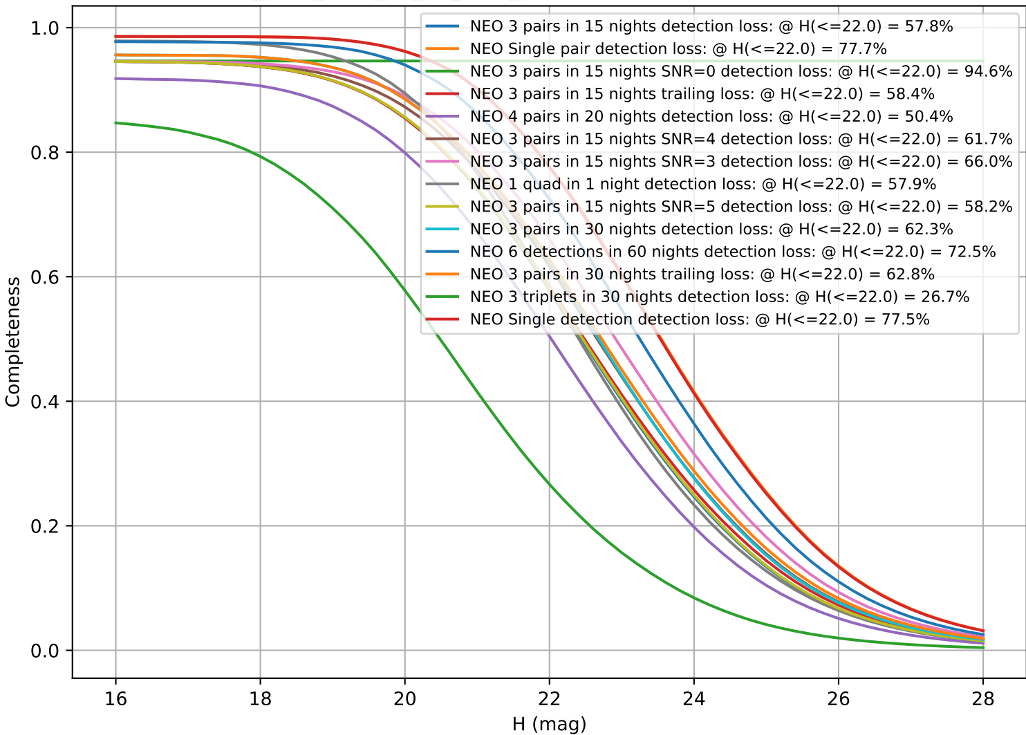
too_elab_r256_d3_gz_v3.4_10yrs: CumulativeCompleteness
