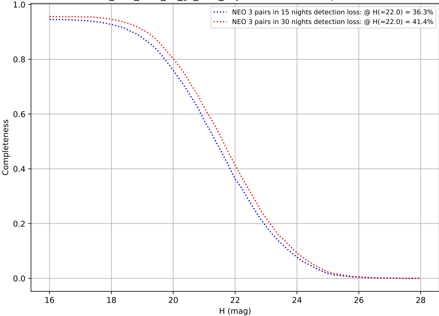
too_elab_r256_d3_gz_v3.4_10yrs: DifferentialCompleteness
