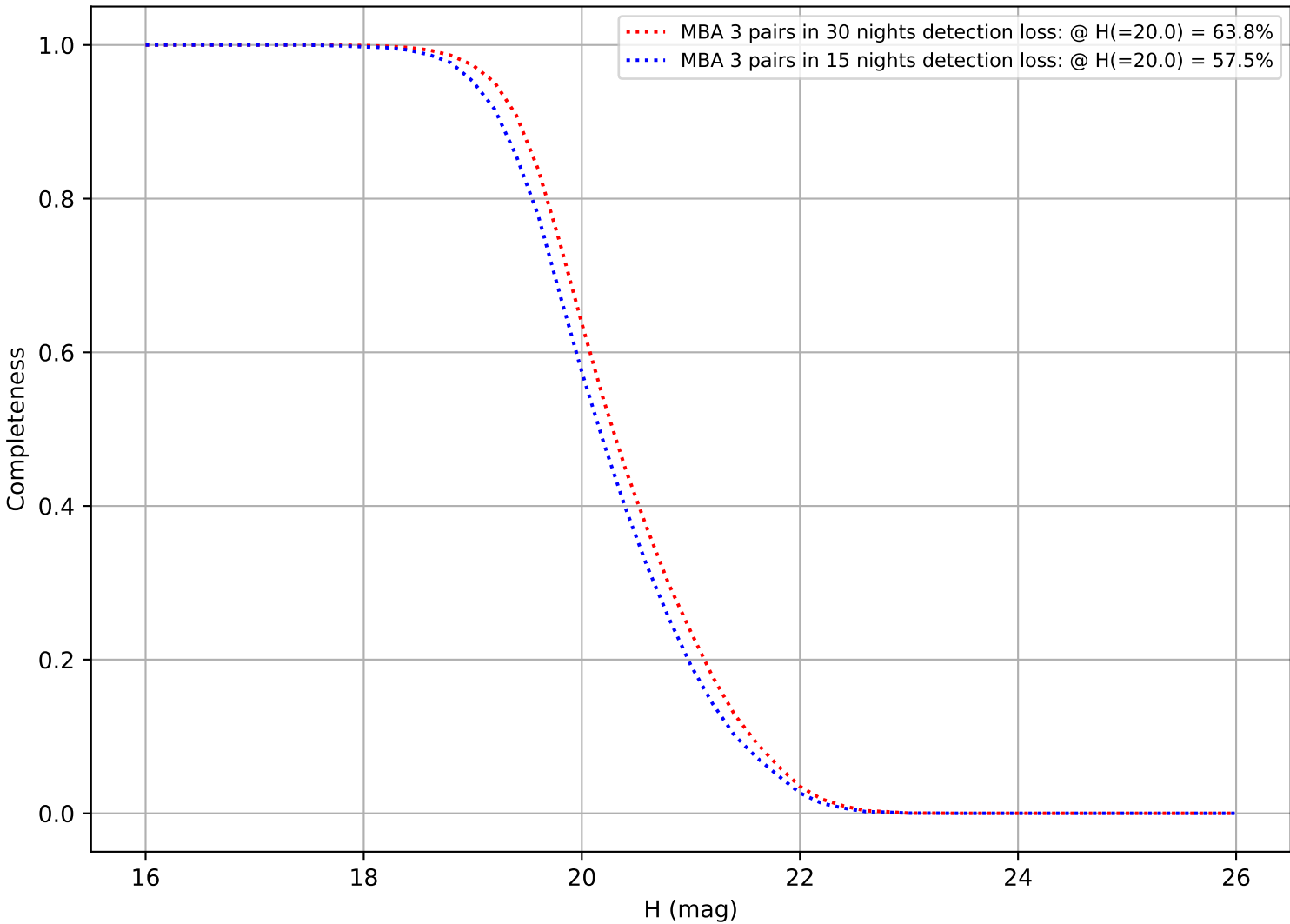
too_elab_r256_d3_gz_v3.4_10yrs: DifferentialCompleteness
