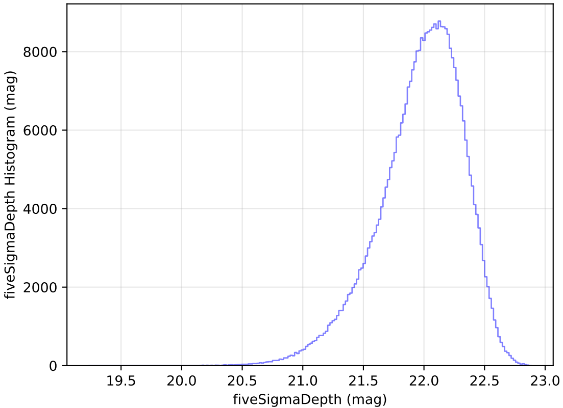
too_elab_r256_d3_gz_v3.4_10yrs y: fiveSigmaDepth Histogram
