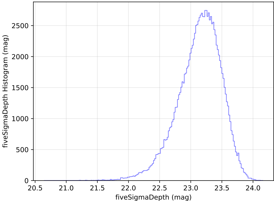
too_elab_r256_d3_gz_v3.4_10yrs u: fiveSigmaDepth Histogram
