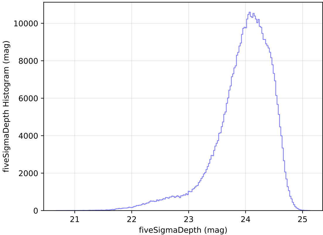
too_elab_r256_d3_gz_v3.4_10yrs r: fiveSigmaDepth Histogram
