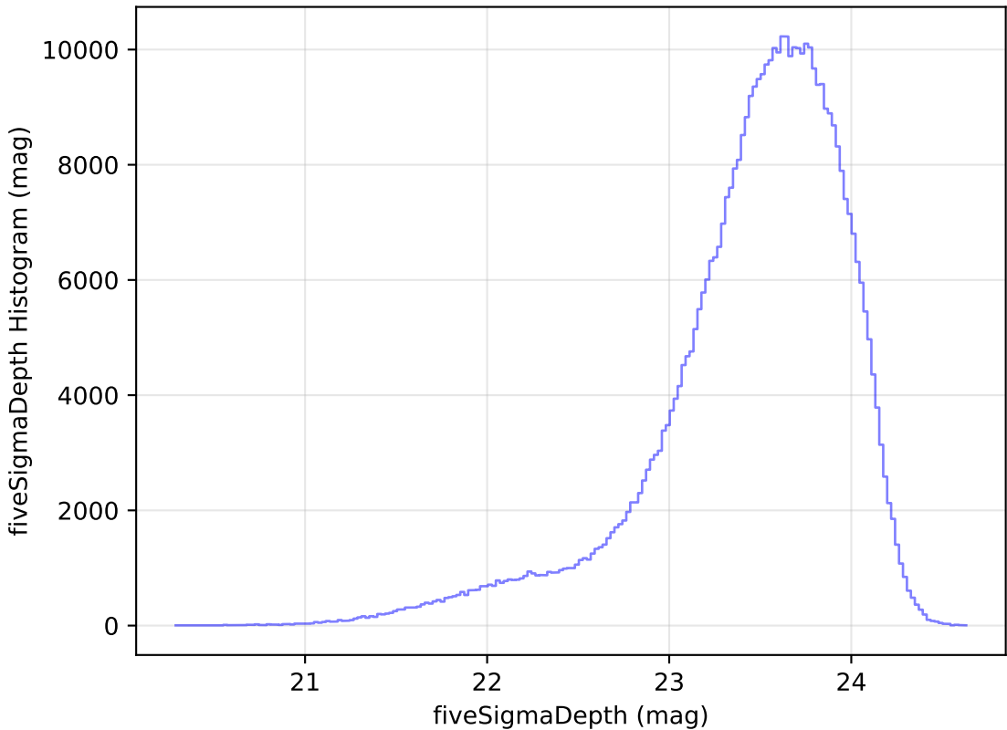
too_elab_r256_d3_gz_v3.4_10yrs i: fiveSigmaDepth Histogram
