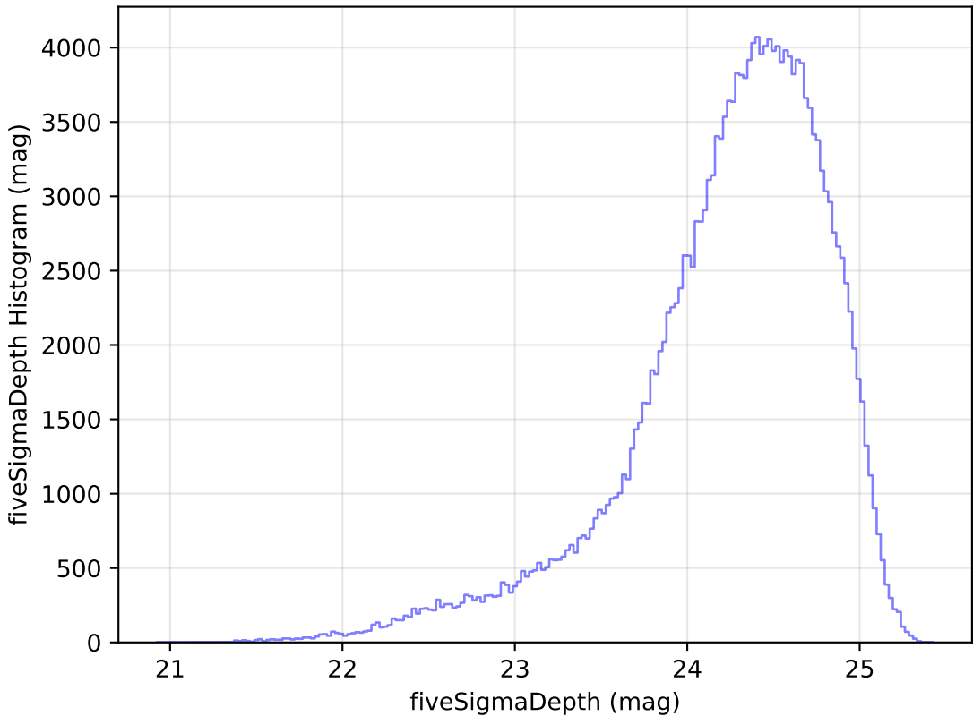
too_elab_r256_d3_gz_v3.4_10yrs g: fiveSigmaDepth Histogram
