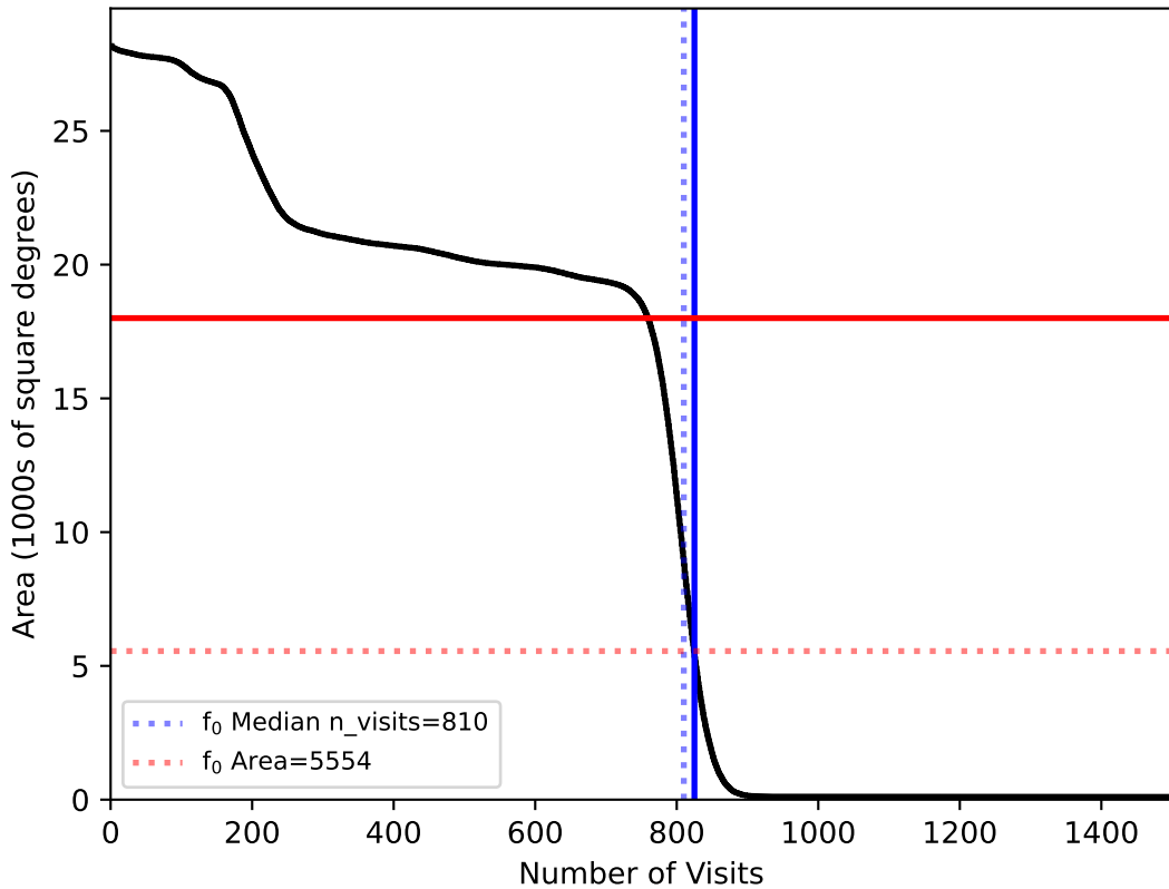
too_elab_r256_d3_gz_v3.4_10yrs : f0
