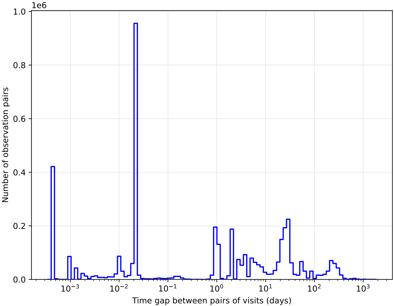
too_elab_r256_d3_gz_v3.4_10yrs y band: Tgaps observationStartMJD
