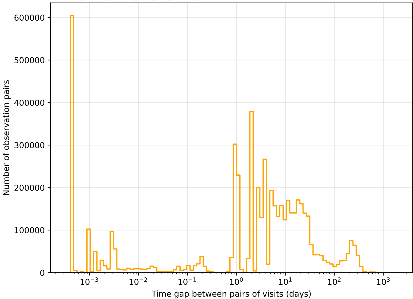
too_elab_r256_d3_gz_v3.4_10yrs r band: Tgaps observationStartMJD
