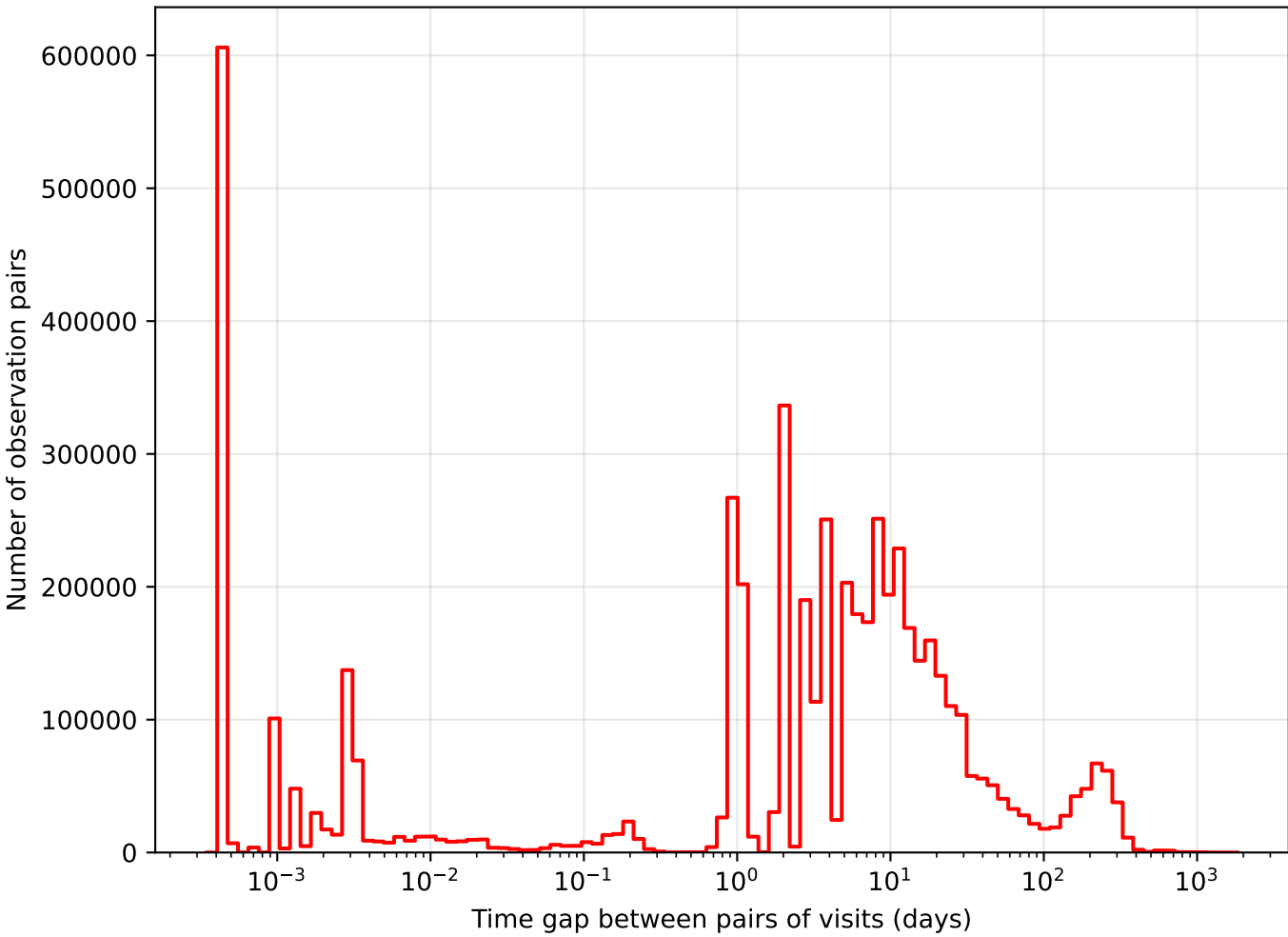
too_elab_r256_d3_gz_v3.4_10yrs i band: Tgaps observationStartMJD
