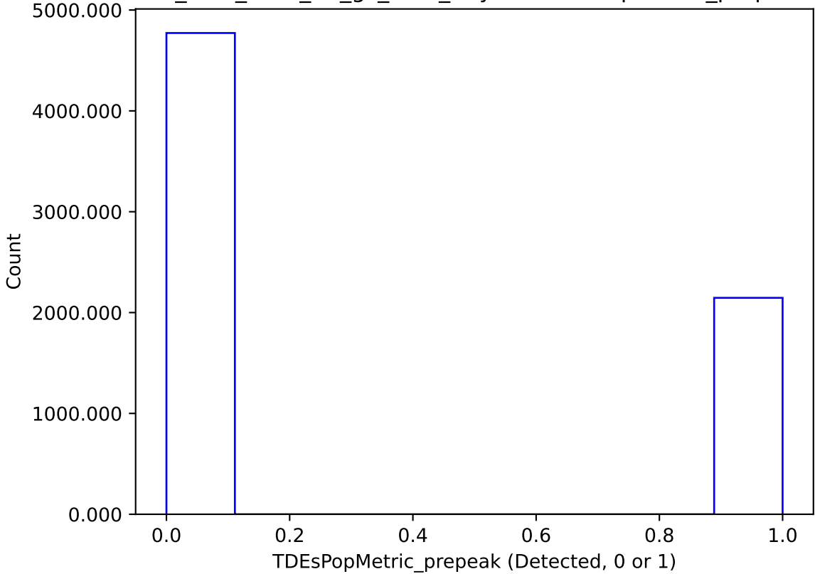
too_elab_r256_d3_gz_v3.4_10yrs : TDEsPopMetric_prepeak
