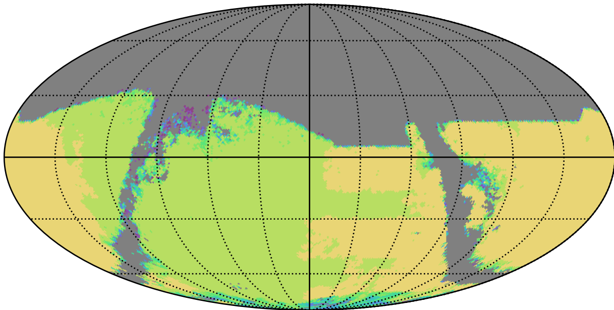
too_elab_r256_d3_gz_v3.4_10yrs : TDC_campaign
