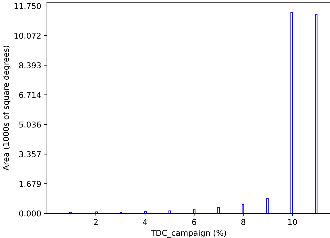
too_elab_r256_d3_gz_v3.4_10yrs : TDC_campaign
