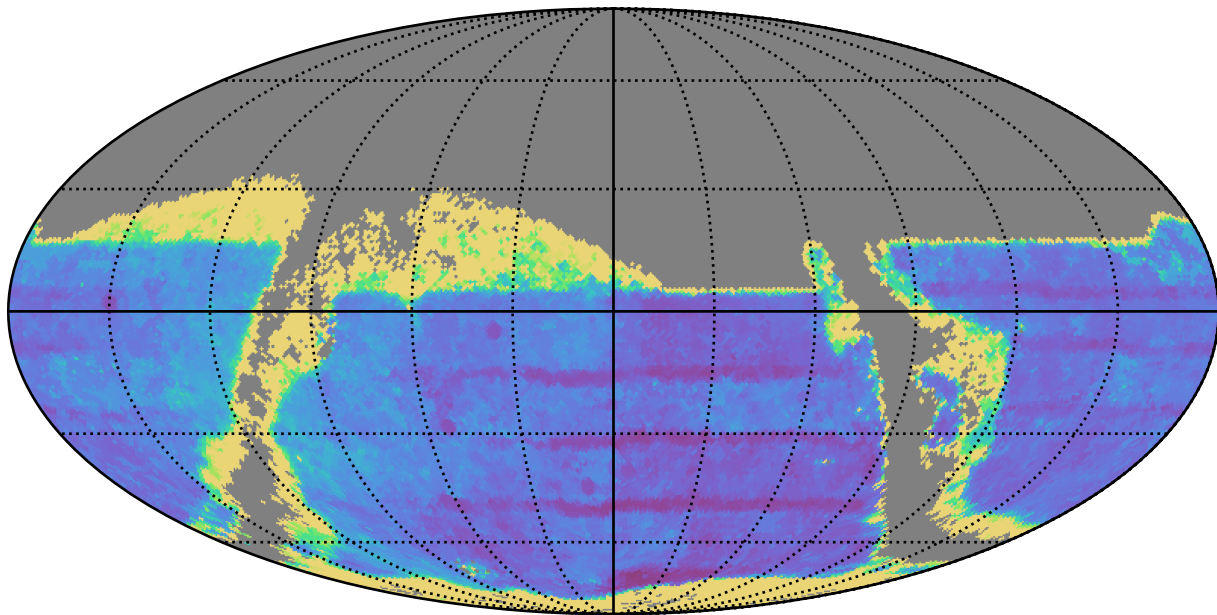
too_elab_r256_d3_gz_v3.4_10yrs : TDC_accuracy
