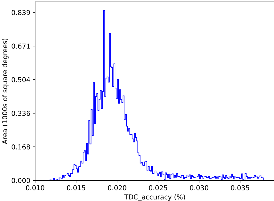
too_elab_r256_d3_gz_v3.4_10yrs : TDC_accuracy
