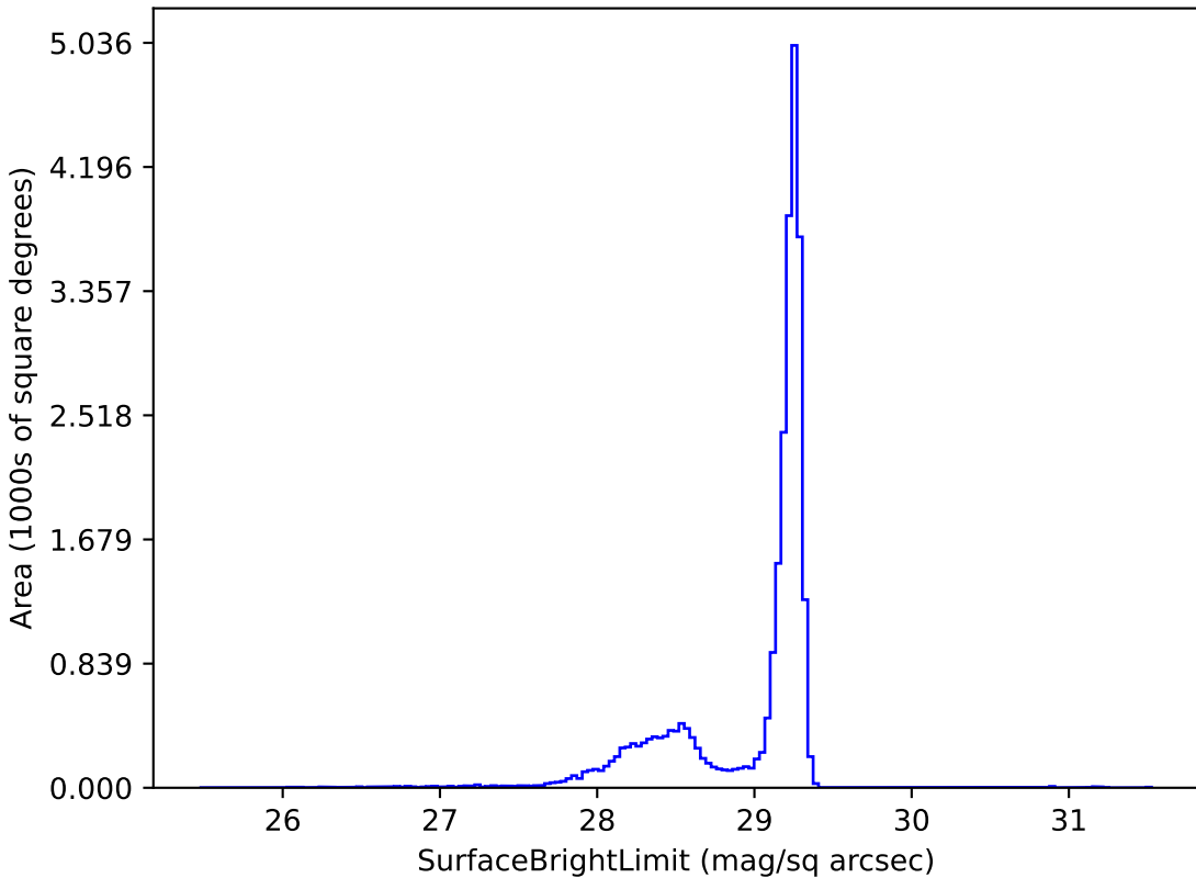
too_elab_r256_d3_gz_v3.4_10yrs z: SurfaceBrightLimit
