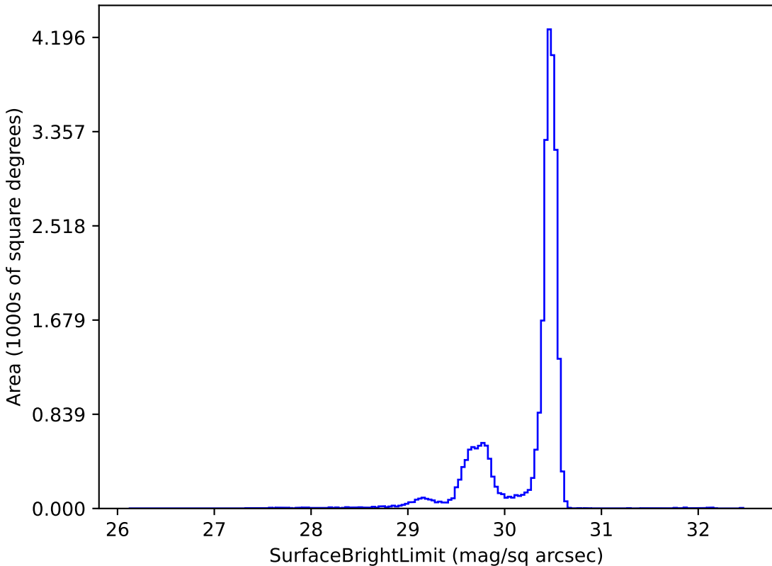
too_elab_r256_d3_gz_v3.4_10yrs r: SurfaceBrightLimit
