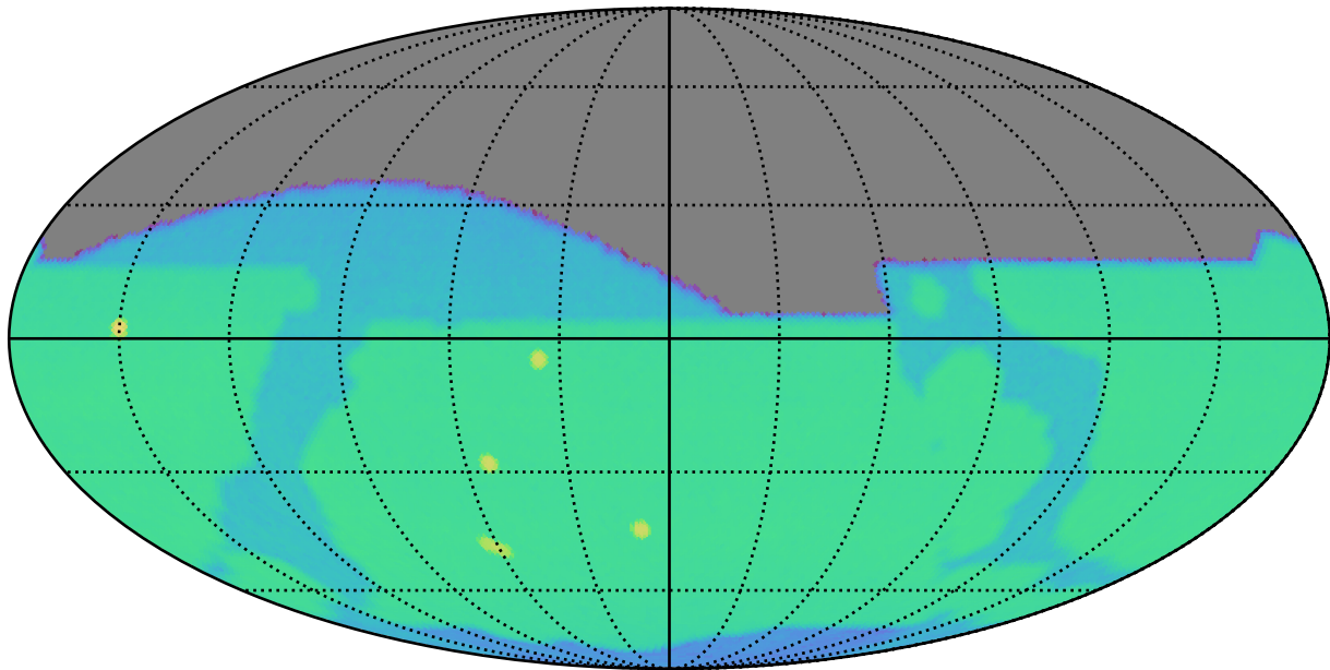
too_elab_r256_d3_gz_v3.4_10yrs i: SurfaceBrightLimit
