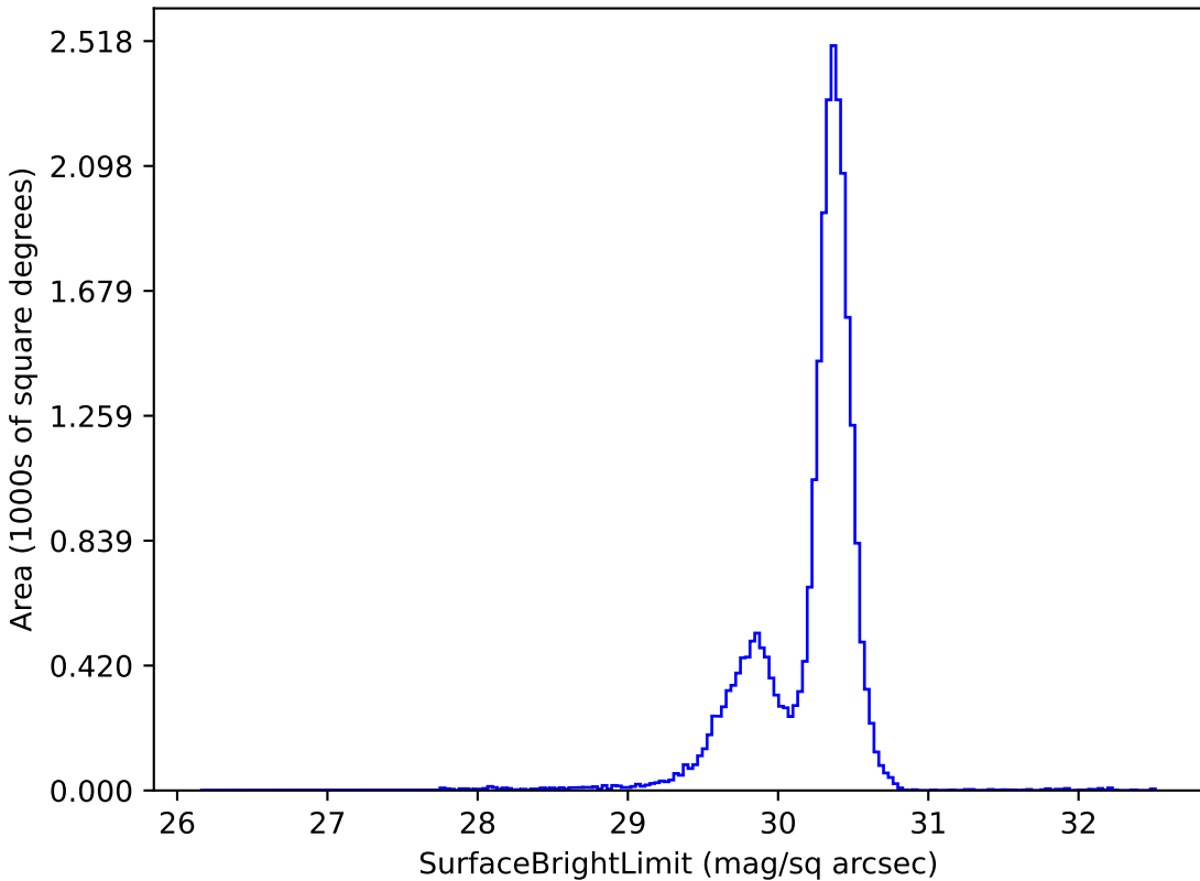
too_elab_r256_d3_gz_v3.4_10yrs g: SurfaceBrightLimit
