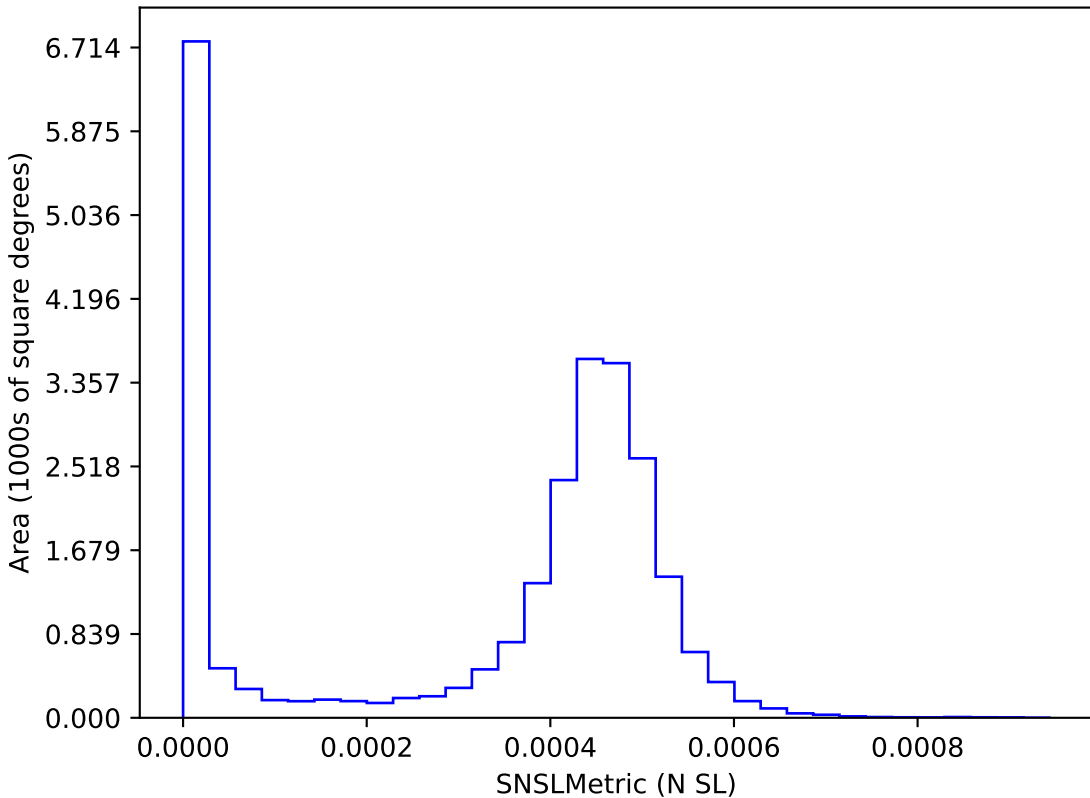
too_elab_r256_d3_gz_v3.4_10yrs : SNSLMetric
