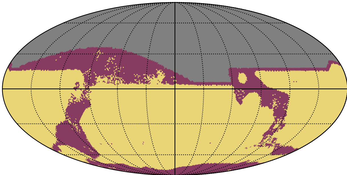
too_elab_r256_d3_gz_v3.4_10yrs : RapidRevisits
