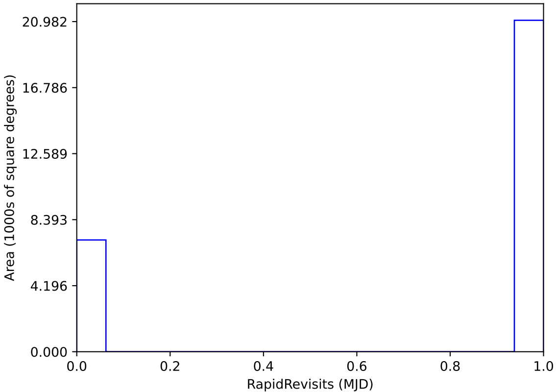
too_elab_r256_d3_gz_v3.4_10yrs : RapidRevisits
