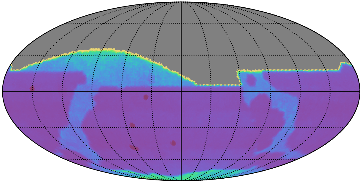
too_elab_r256_d3_gz_v3.4_10yrs : Proper Motion Uncert @ 20.5
