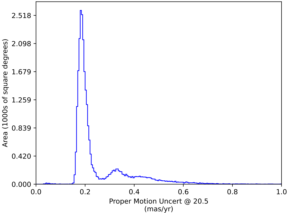
too_elab_r256_d3_gz_v3.4_10yrs : Proper Motion Uncert @ 20.5
