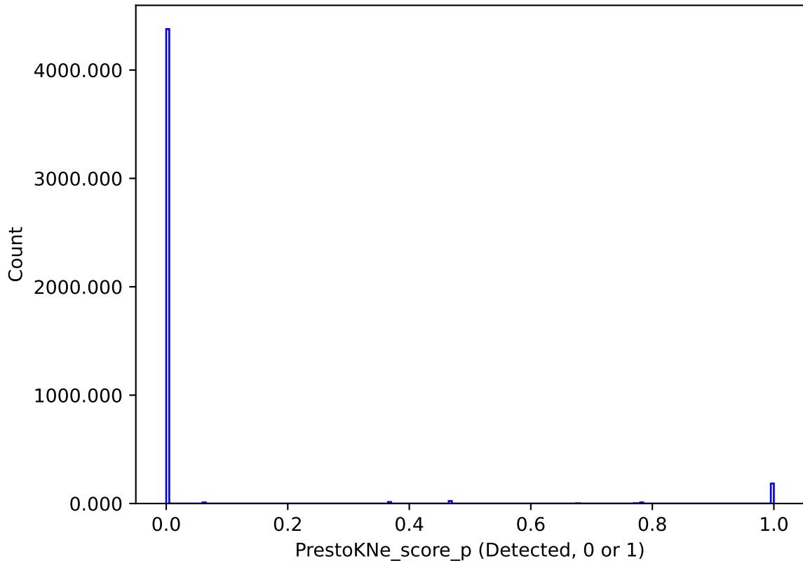
too_elab_r256_d3_gz_v3.4_10yrs : PrestoKNe_score_p
