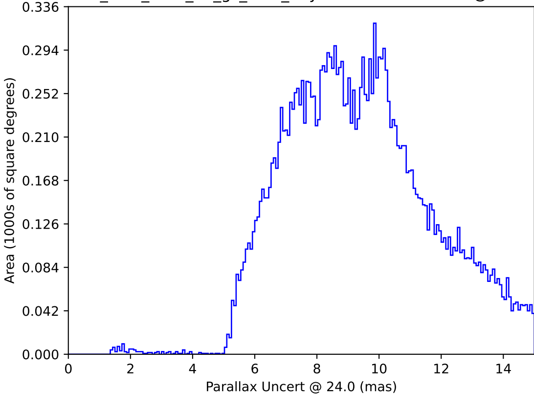
too_elab_r256_d3_gz_v3.4_10yrs : Parallax Uncert @ 24.0
