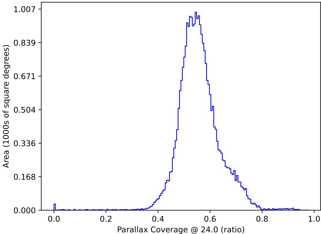
too_elab_r256_d3_gz_v3.4_10yrs : Parallax Coverage @ 24.0
