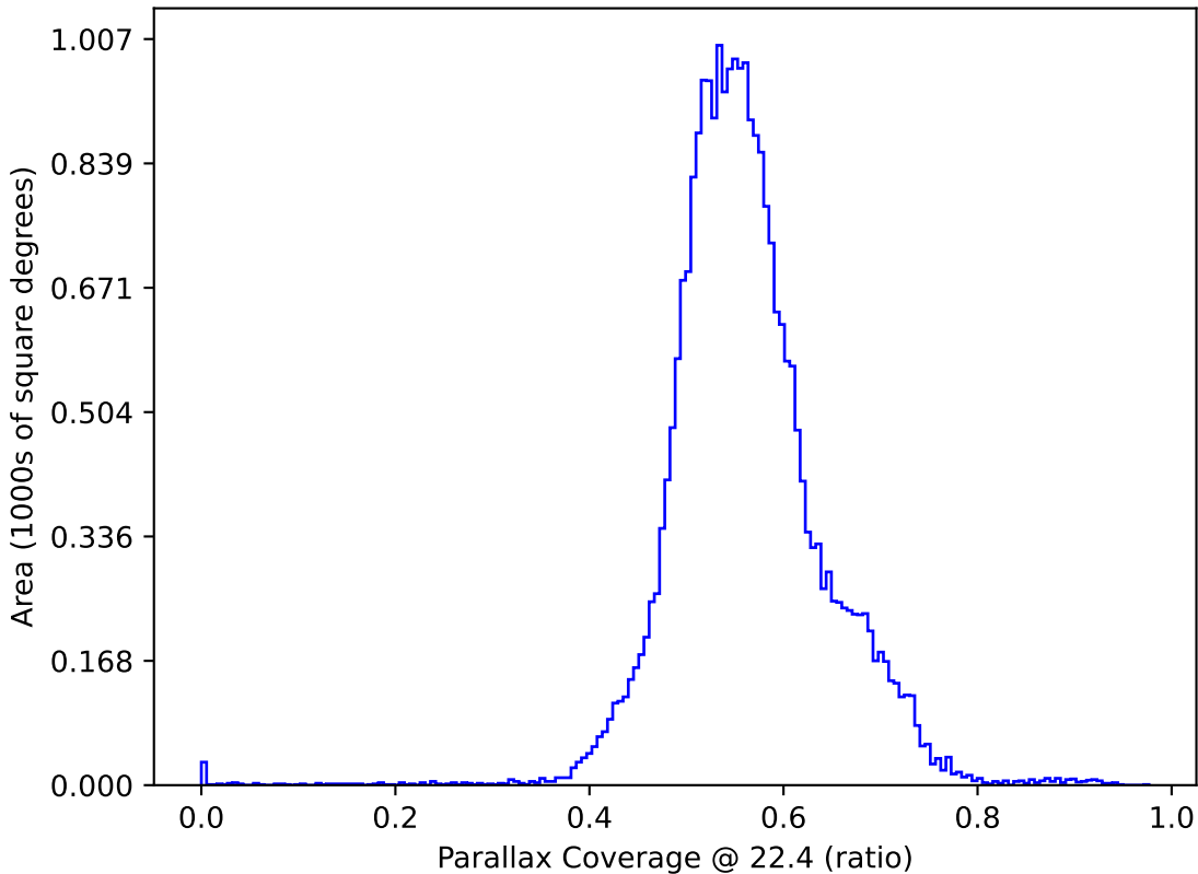
too_elab_r256_d3_gz_v3.4_10yrs : Parallax Coverage @ 22.4
