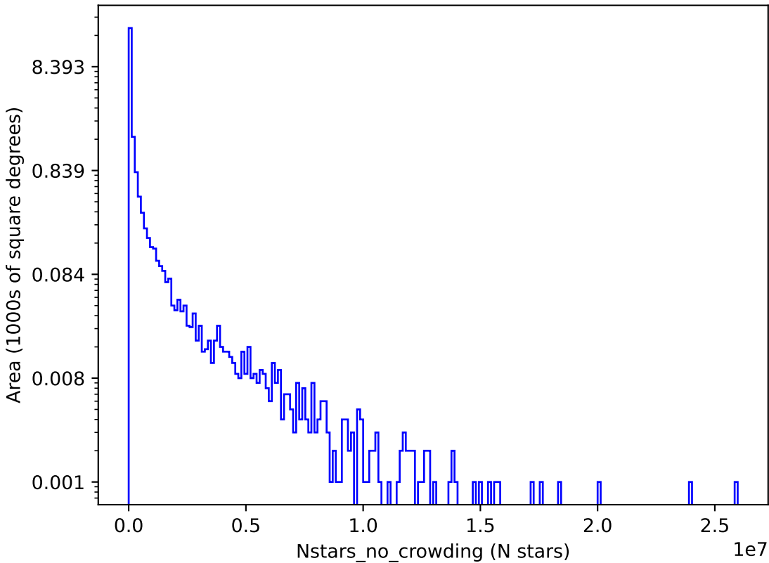
too_elab_r256_d3_gz_v3.4_10yrs y: Nstars_no_crowding
