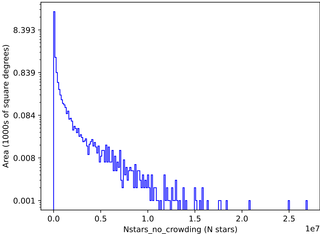
too_elab_r256_d3_gz_v3.4_10yrs i: Nstars_no_crowding
