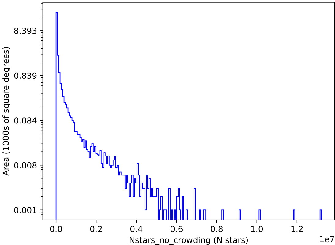
too_elab_r256_d3_gz_v3.4_10yrs g: Nstars_no_crowding
