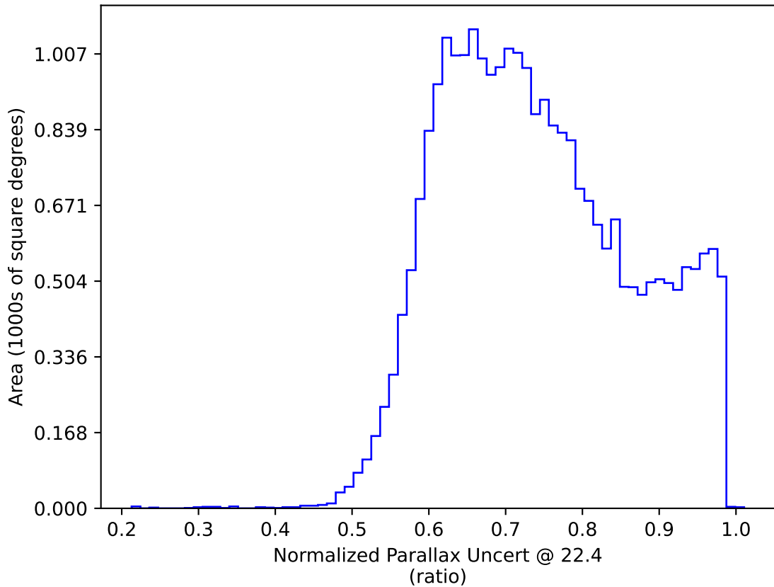
too_elab_r256_d3_gz_v3.4_10yrs : Normalized Parallax Uncert @ 22.4
