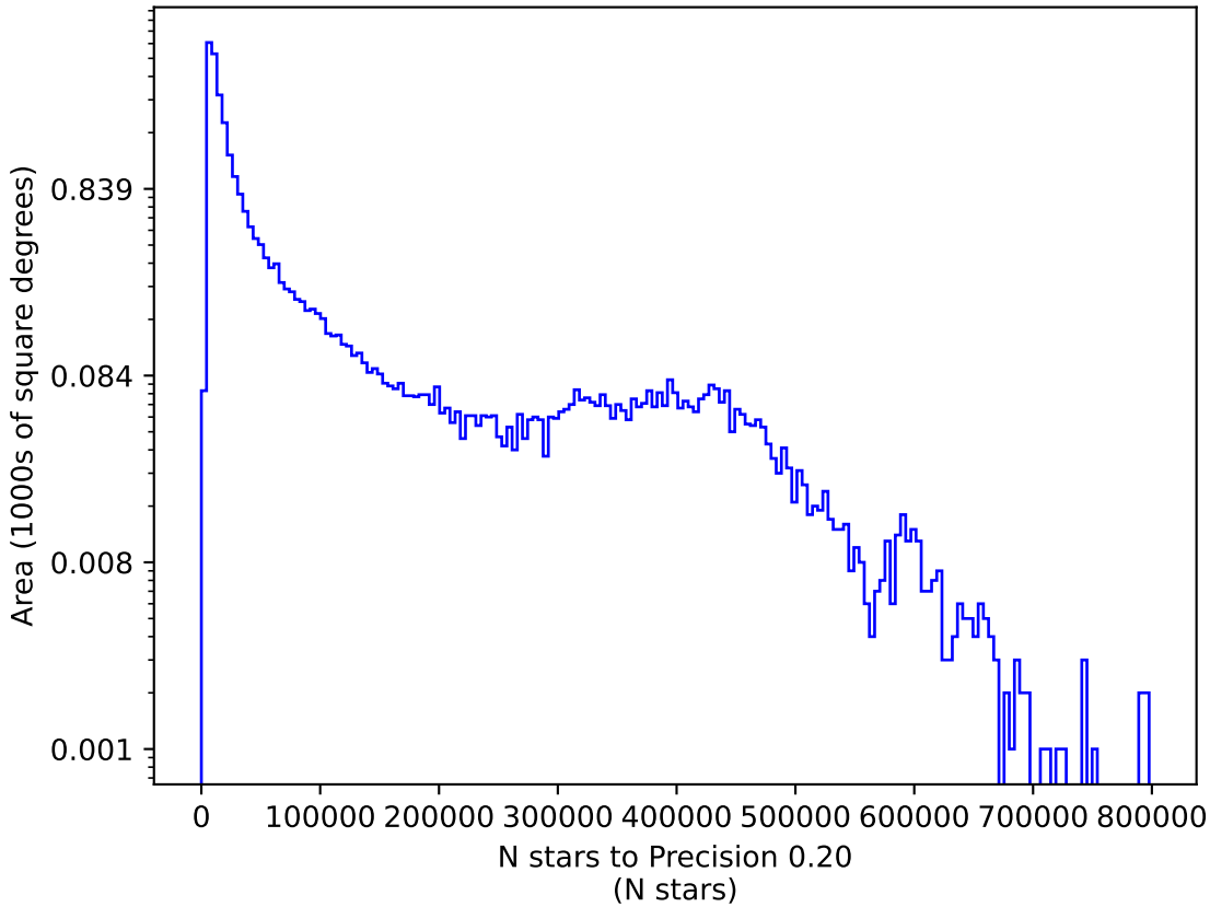
too_elab_r256_d3_gz_v3.4_10yrs r: N stars to Precision 0.20
