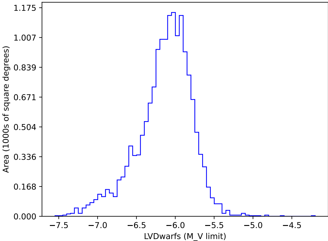
too_elab_r256_d3_gz_v3.4_10yrs gi: LVDwarfs
