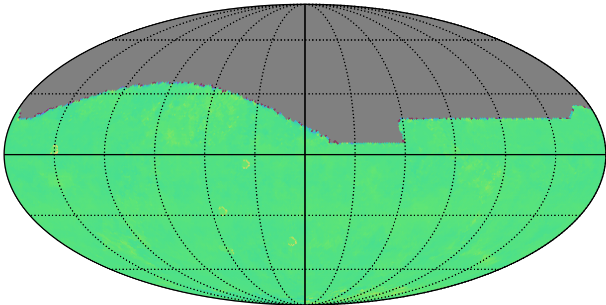
too_elab_r256_d3_gz_v3.4_10yrs r: Kuiper rotTelPos
