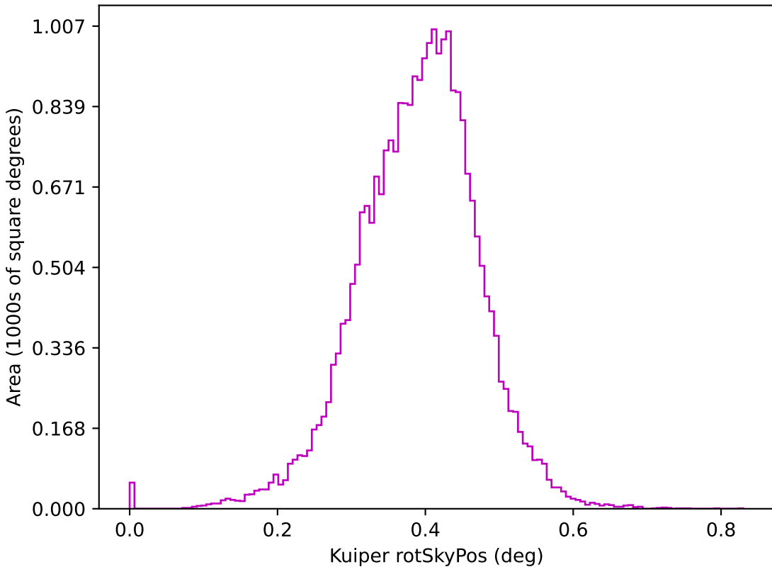
too_elab_r256_d3_gz_v3.4_10yrs z: Kuiper rotSkyPos
