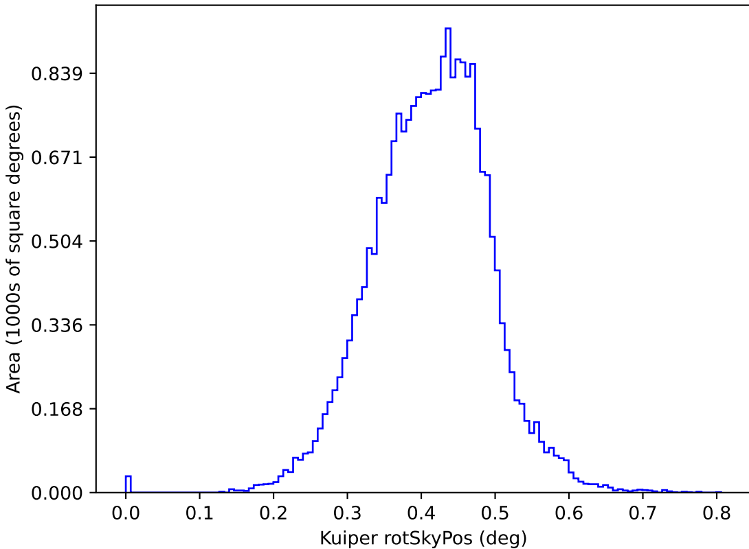
too_elab_r256_d3_gz_v3.4_10yrs y: Kuiper rotSkyPos
