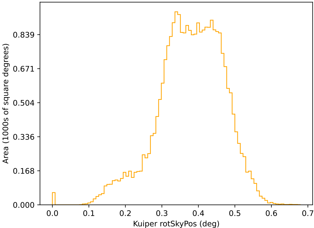
too_elab_r256_d3_gz_v3.4_10yrs r: Kuiper rotSkyPos
