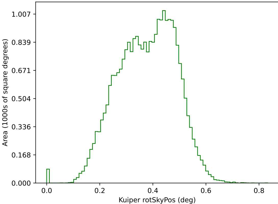
too_elab_r256_d3_gz_v3.4_10yrs g: Kuiper rotSkyPos
