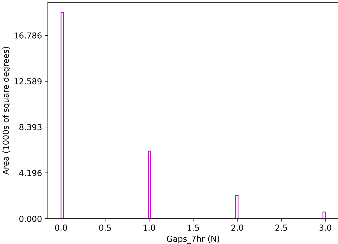
too_elab_r256_d3_gz_v3.4_10yrs z band: Gaps_7hr
