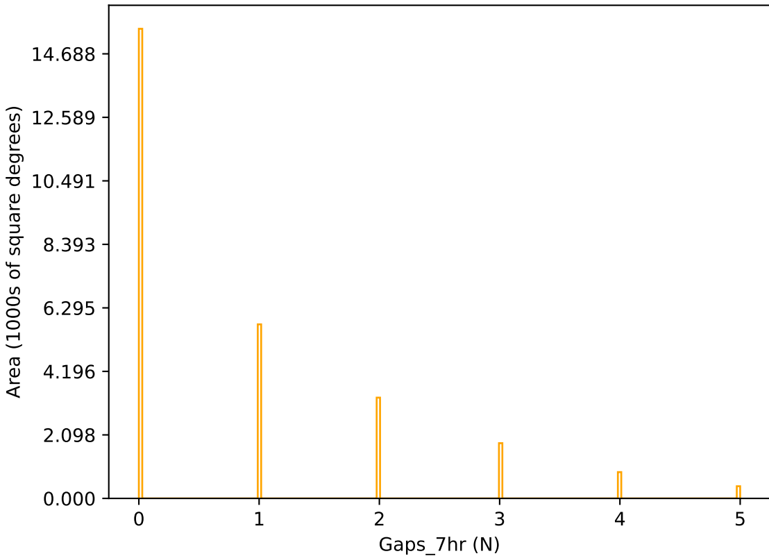
too_elab_r256_d3_gz_v3.4_10yrs r band: Gaps_7hr
