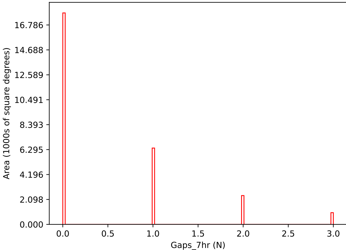
too_elab_r256_d3_gz_v3.4_10yrs i band: Gaps_7hr
